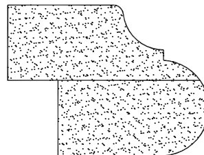
1-1/2" Roman Ogee Bullnose (Laminated)
